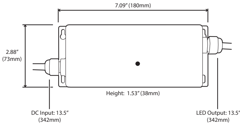
CONTROLLER TOP
